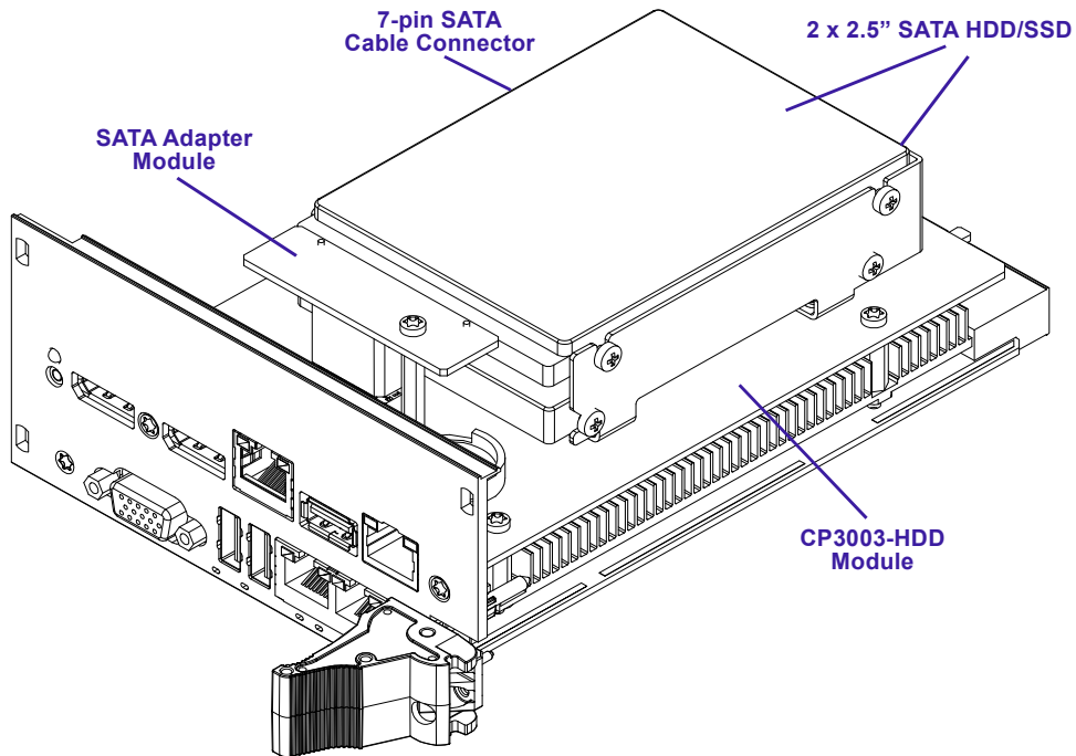
Figure 3-4: 12 HP CP3003-SA with CP3003-HDD Module and SATA Adapter Module
