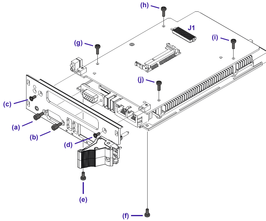
Figure 3-7: Screws Securing the XMC Module to the CP3003-XMC Extension Module
