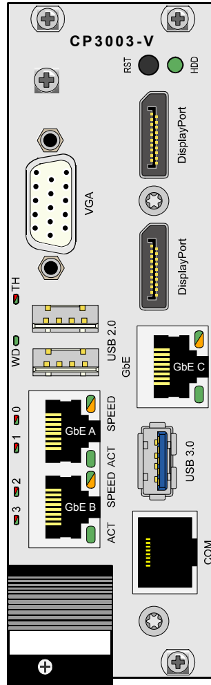
Figure F-2: Front Panel of the CP3003-V
