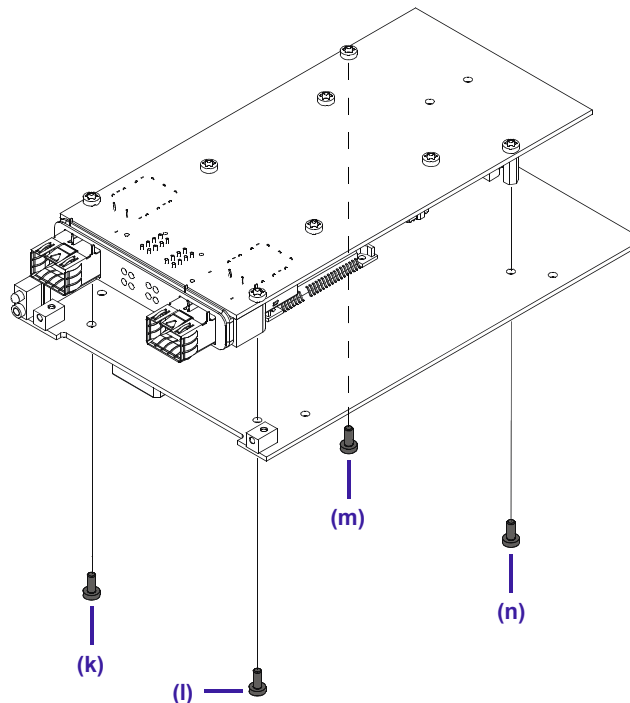
Figure 3-7: Screws Securing the XMC Module to the CP3003-XMC Extension Module
