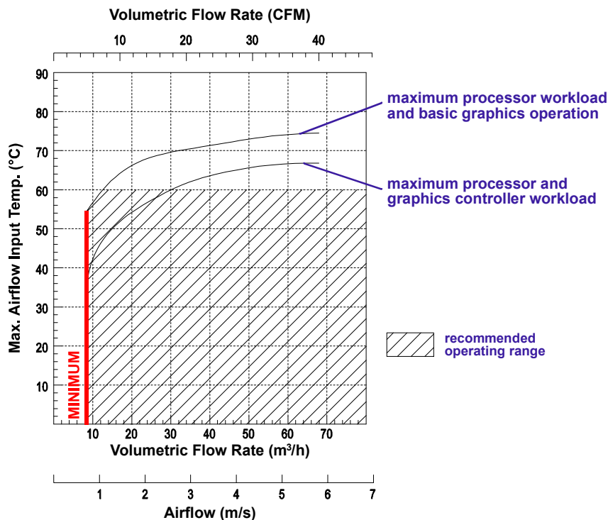
Figure 6-1: CP3003-SA with i7-3612QE (SV), 2.1 GHz
