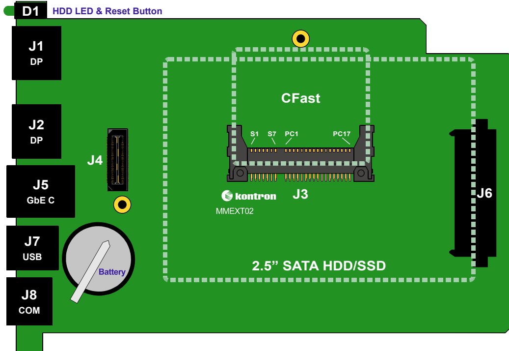
Figure A-3: CP3003-HDD Module Layout for 8 HP Board Version (Top View)
