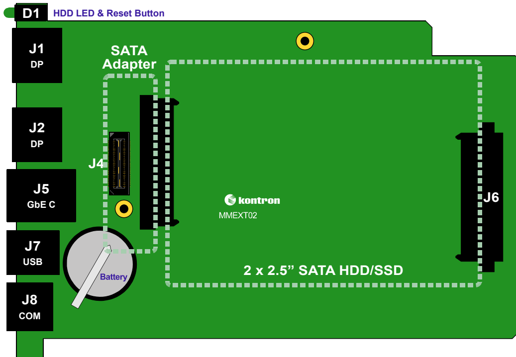
Figure A-4: CP3003-HDD Module Layout for 12 HP Board Version (Top View)
