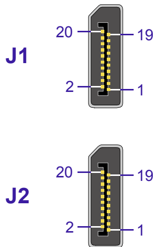
Figure A-6: DisplayPort Connectors J1 and J2
