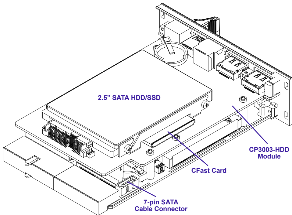
Figure 3-3: 8 HP CP3003-SA with CP3003-HDD Module
