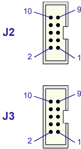
Figure C-8: Serial Port Connectors J2 (COMA) and J3 (COMB)
