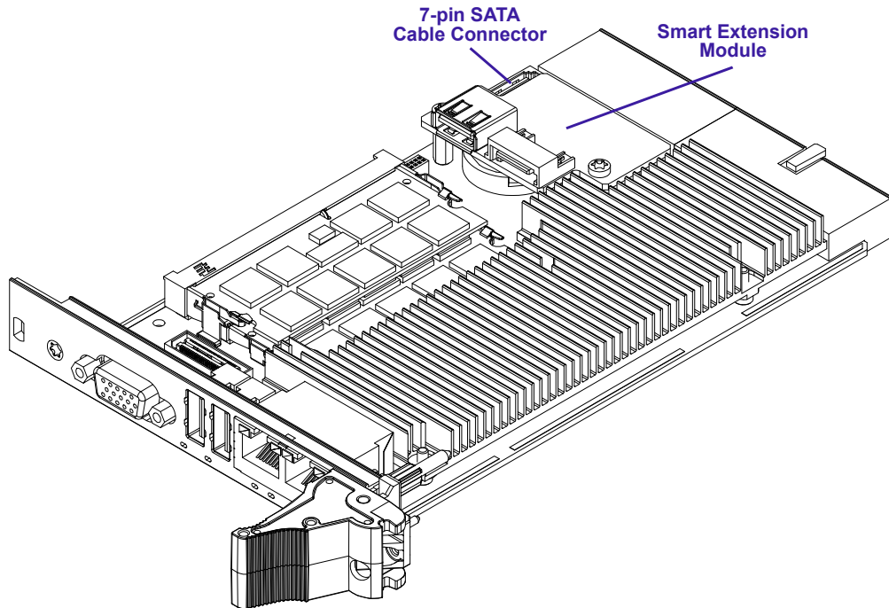
Figure 3-2: 4 HP CP3003-SA with Smart Extension Module
