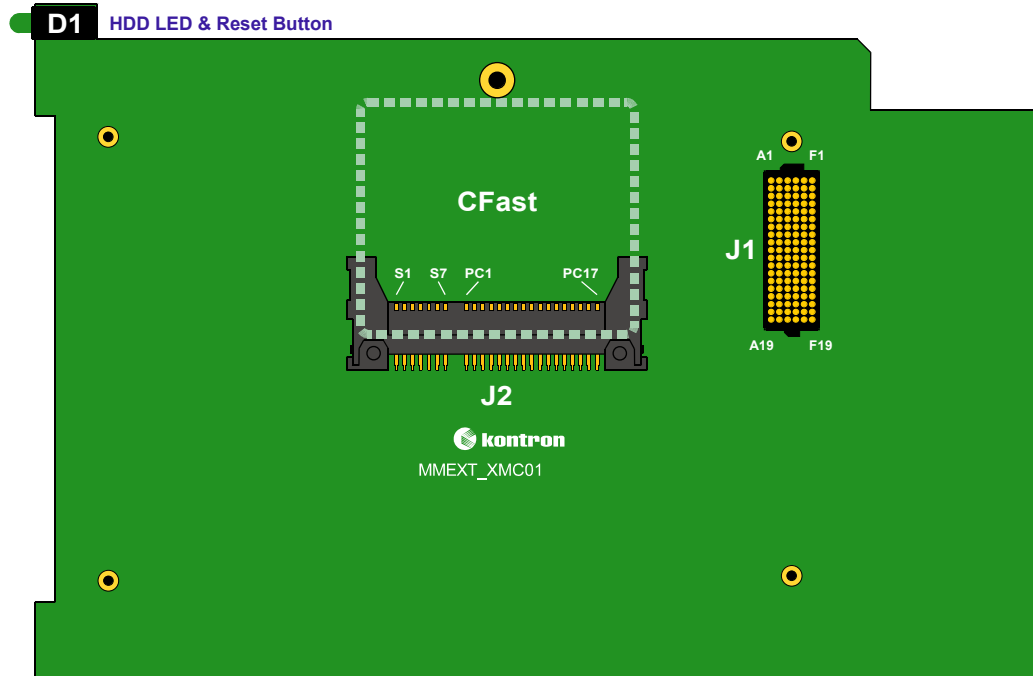
Figure B-3: CP3003-XMC Module Layout (Top View)
