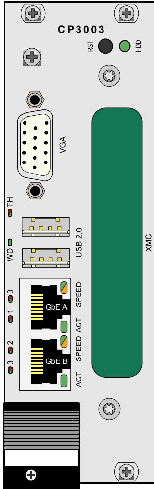
Figure B-2: Front Panel of the 8 HP CP3003-SA with CP3003-XMC Module
