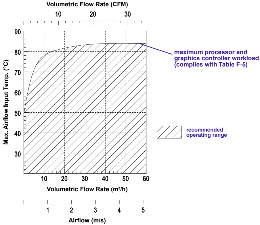
Figure F-3: CP3003-V with Celeron® 807UE, 1.0 GHz
