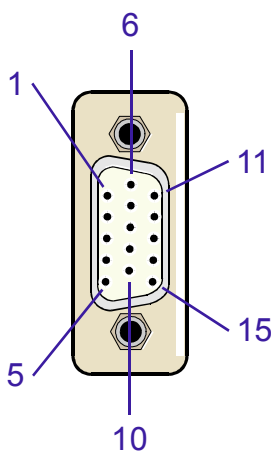
Figure C-5: D-Sub VGA Connector J7 Table C-3: D-Sub VGA Connector J7 Pinout
