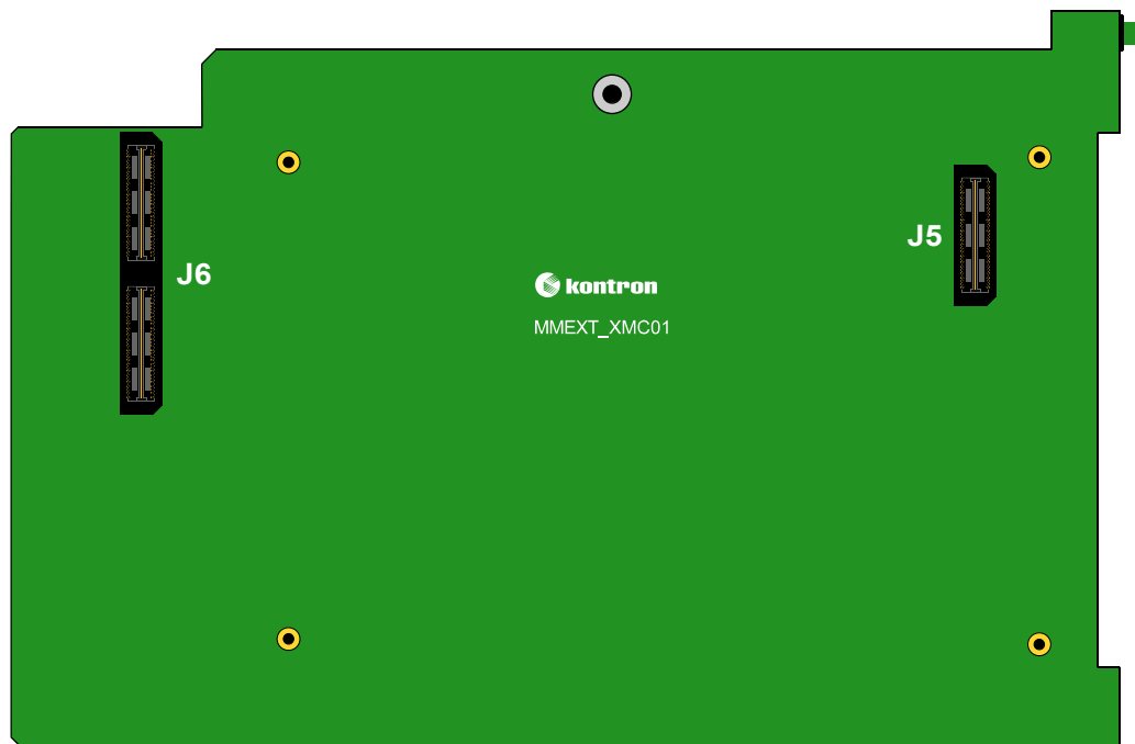
Figure B-4: CP3003-XMC Module Layout (Bottom View)
