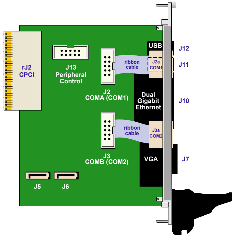
Figure C-3: CP-RIO3-04 Rear I/O Module Layout, 8 HP Version
