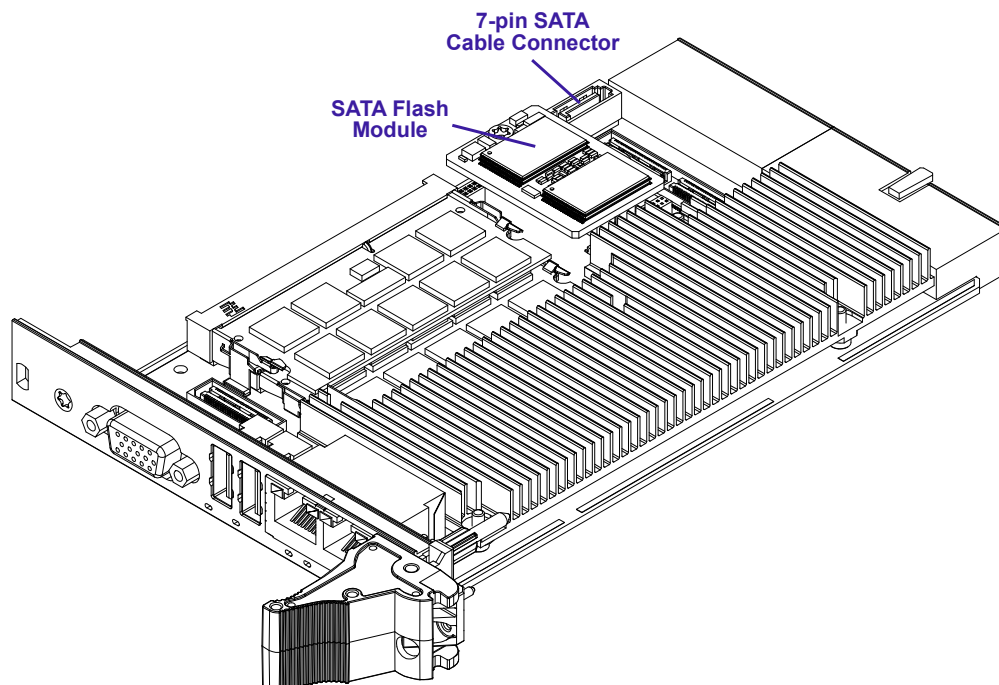
Figure 3-1: 4 HP CP3003-SA with SATA Flash Module
