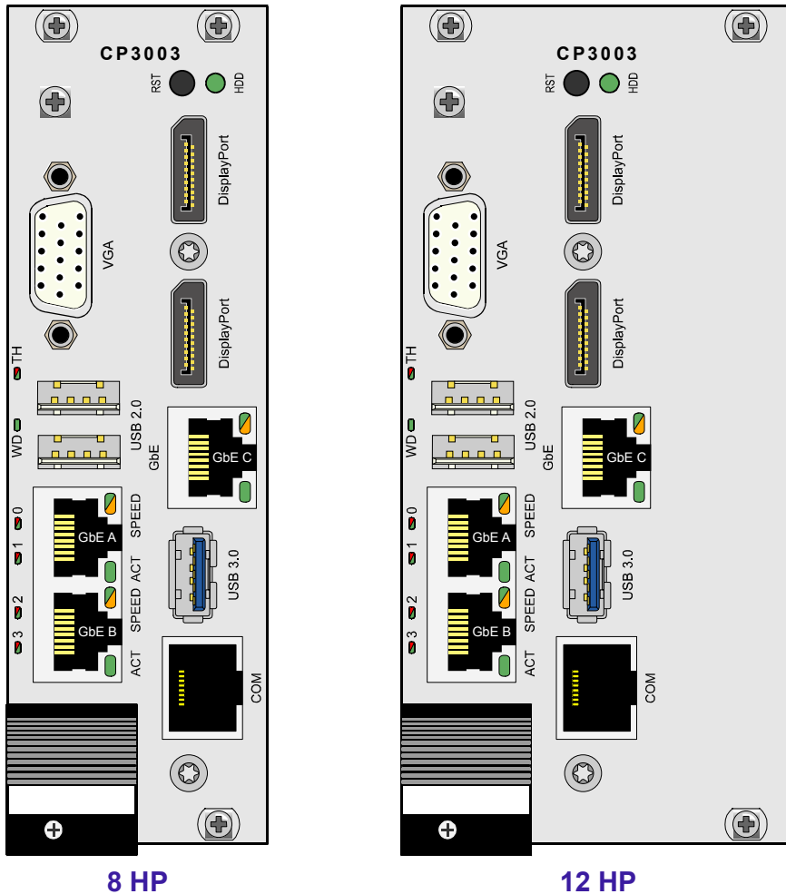
Figure A-2: Front Panel of the 8 HP and 12 HP CP3003-SA with CP3003-HDD Module
