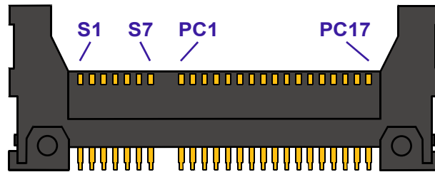
Figure A-10: CFast Connector J3
