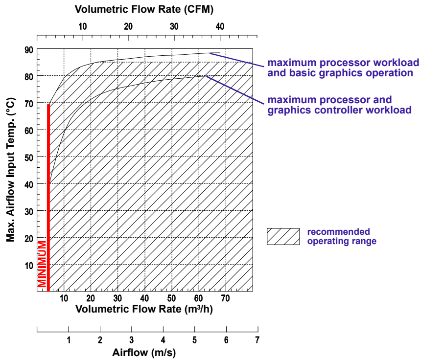
Figure 6-3: CP3003-SA with i7-3517UE (ULV), 1.7 GHz
