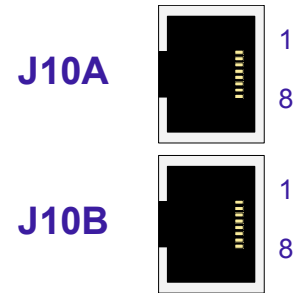
Figure C-6: Dual Gigabit Ethernet Connector J10A/B
