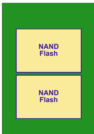
Figure D-1: SATA Flash Module Layout (Top View)
