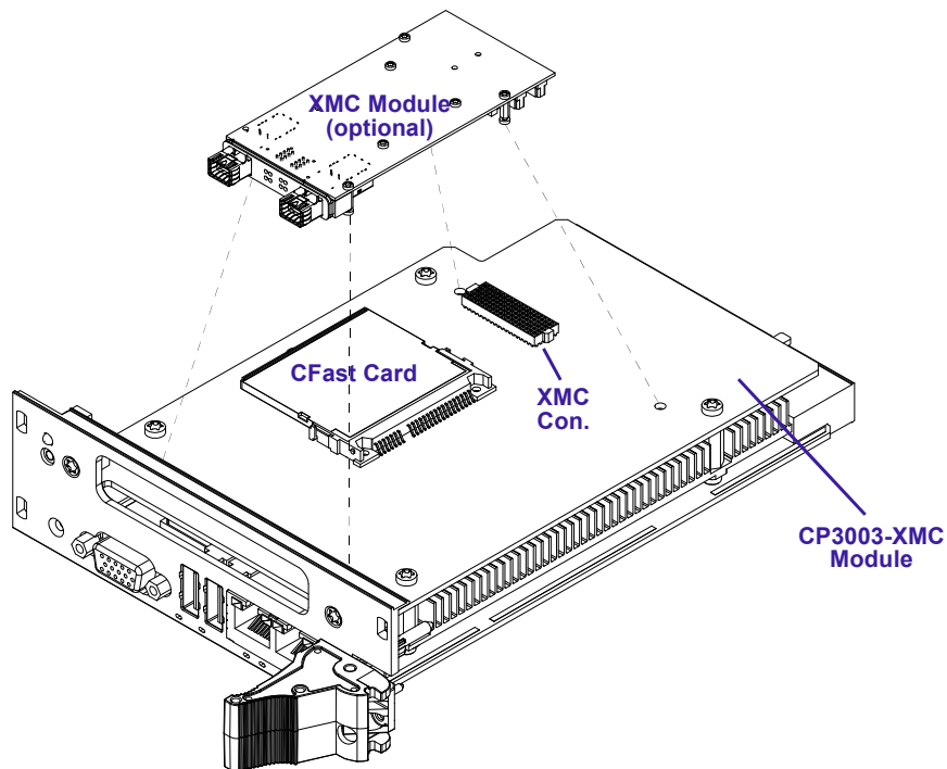
Figure 3-5: 8 HP CP3003-SA with CP3003-XMC Module
