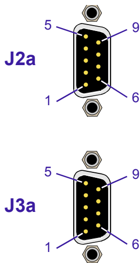
Figure C-7: COM Connectors J2a (COMA) and J3a (COMB) Table C-5: COM Connectors J2a (COMA) and J3a (COMB) Pinout
